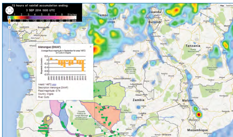
Figure 4: Namibia Flood Dashboard integrates satellite- and ground-data products for user analysis.
