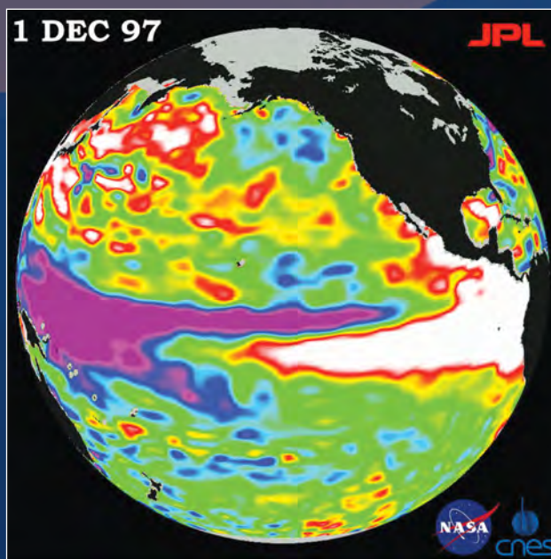
The 1997 El Niño observed by TOPEX/Poseidon
