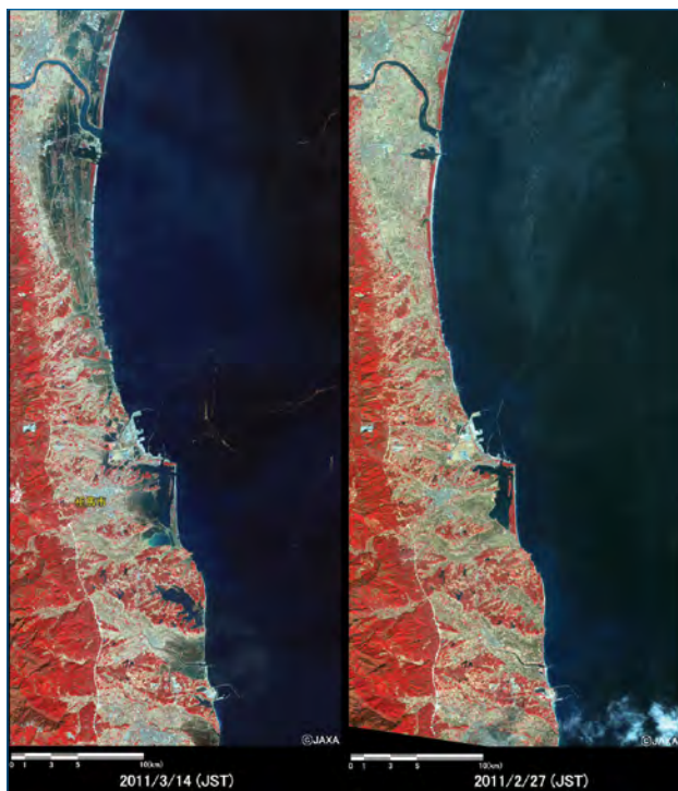
Figure 4: These images from JAXA's ALOS radar satellite were taken before (right) and after (left) the Great East Japan Earthquake and subsequent Tsunami. Areas flooded by water appear dark blue in the post-disaster image.
