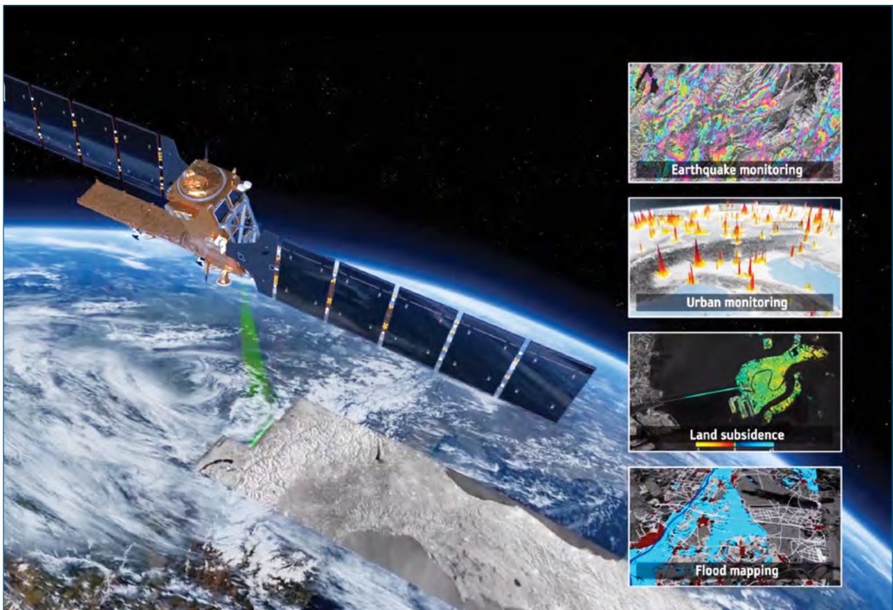
Figure 1: Risk information produced from Sentinel-1 radar data
